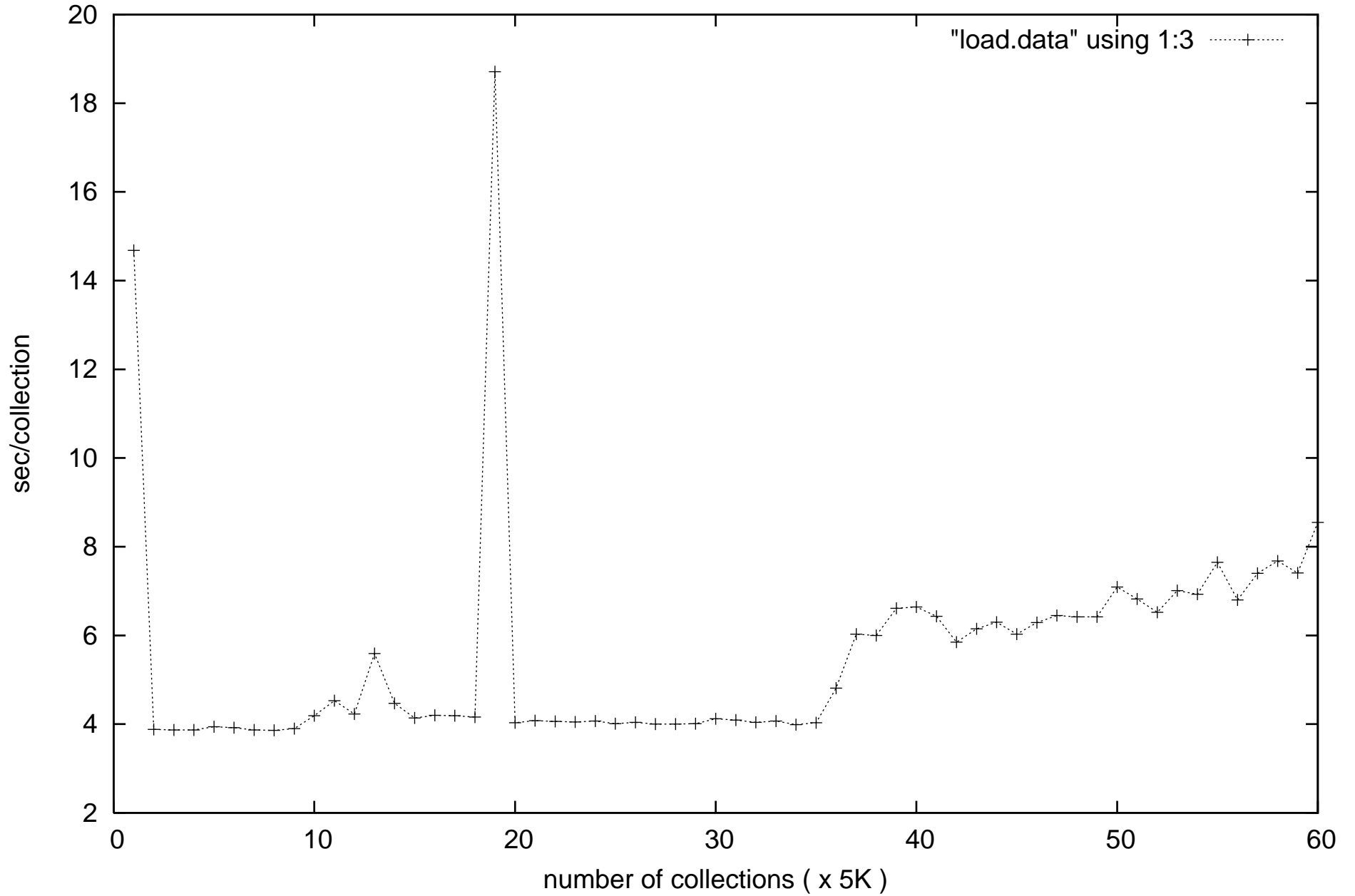
Loading Time Plot for 1 collection
