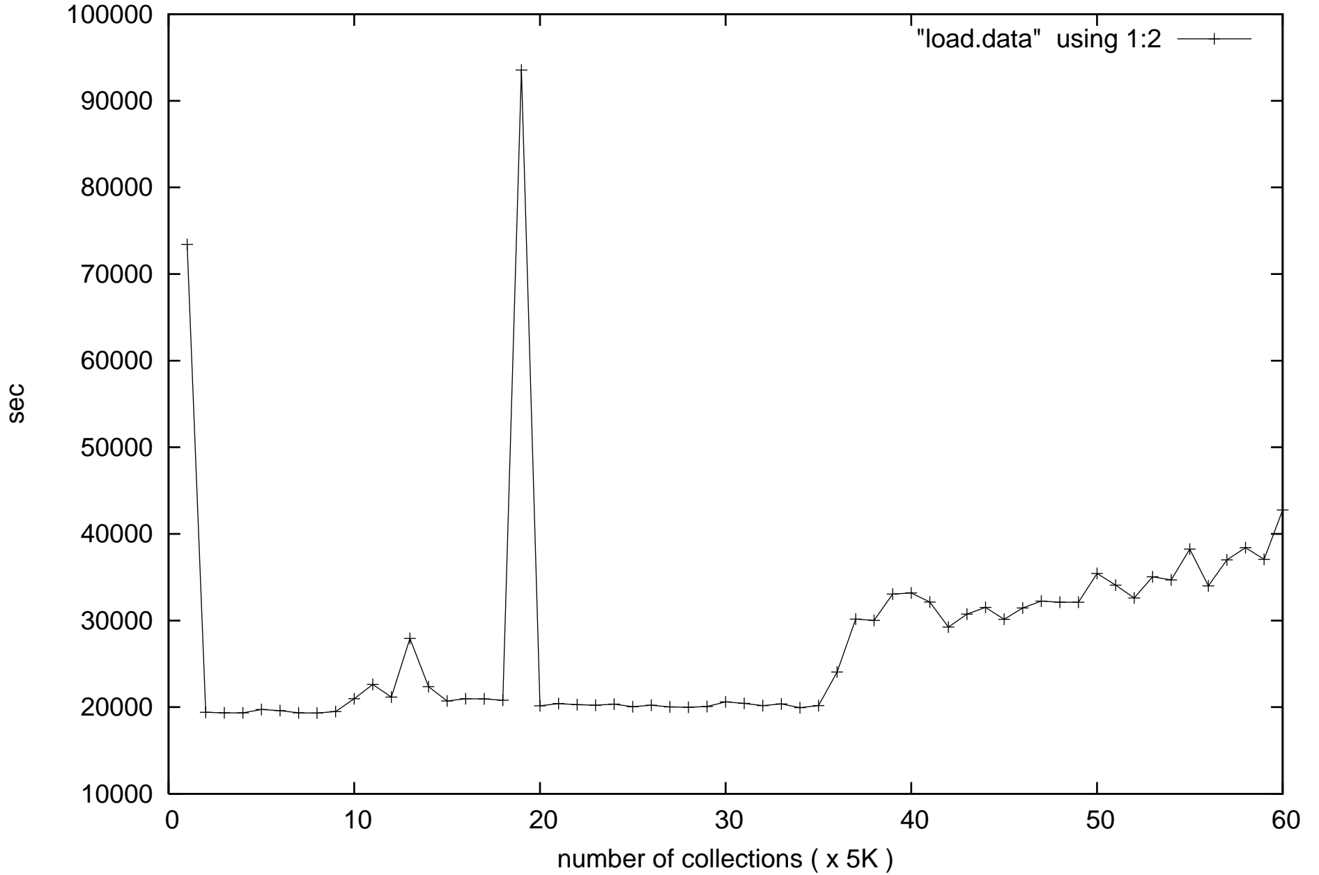
Loading Time Plot for every 5K Collections
