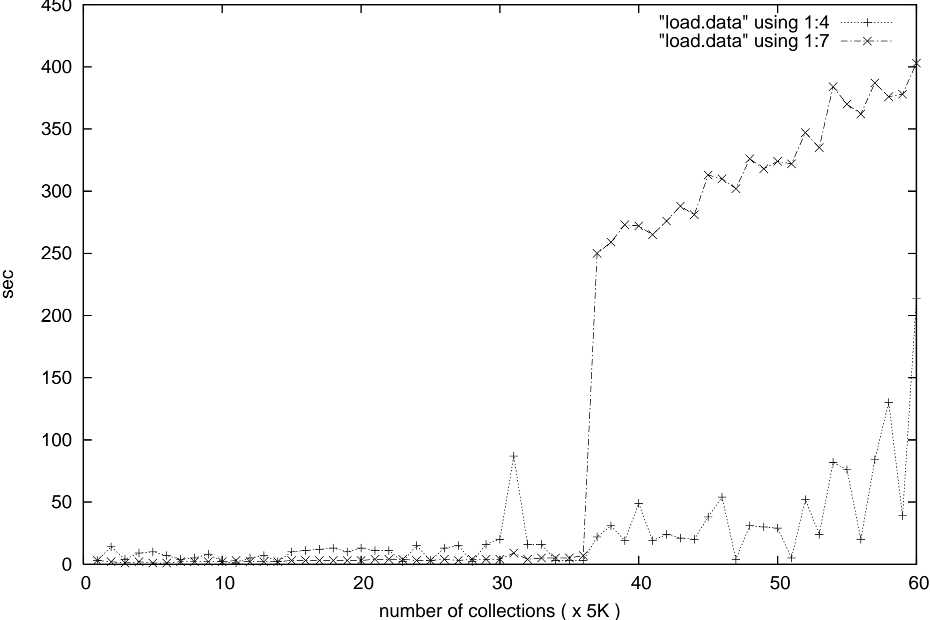
Loading Time Plot for 1 collection and a set of collections
